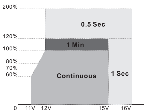
Figure 1 : Output power VS input voltage
