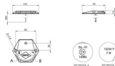
Lampa ostrzegawcza na windę, diodowa 7W 12/24V HOR 80 [LDO 2135] Warning LED light for tail lift, 7W 12/24V HOR 80 [LDO 2135]
